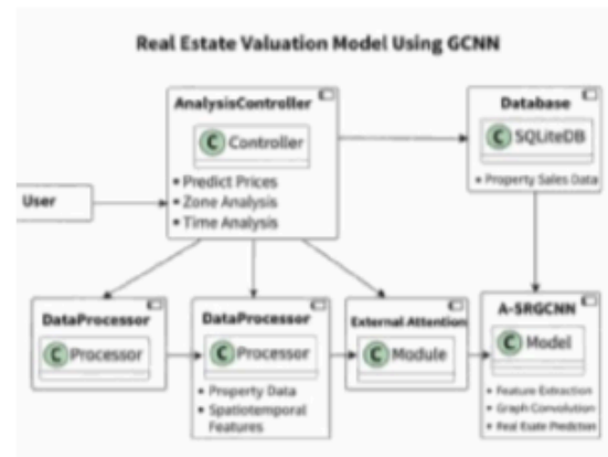
Fig. 6. Component Diagram.
