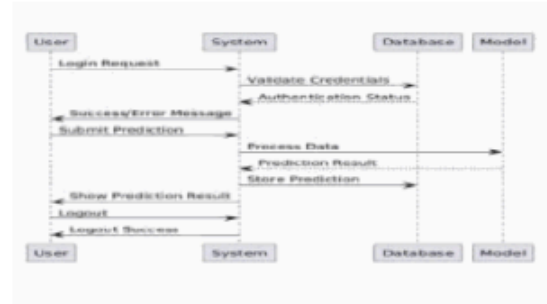
Fig. 5. Sequence Diagram.
